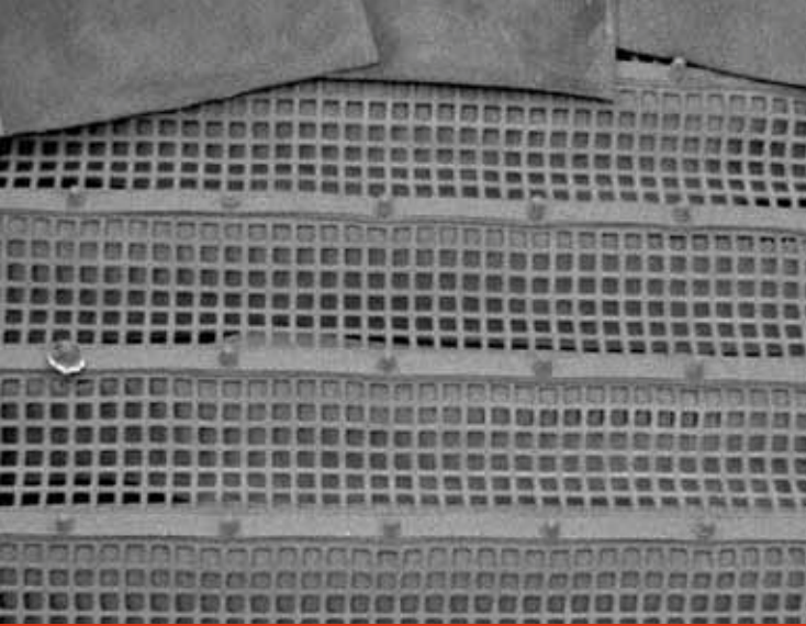
Screen mat for Flipflow screen machine
